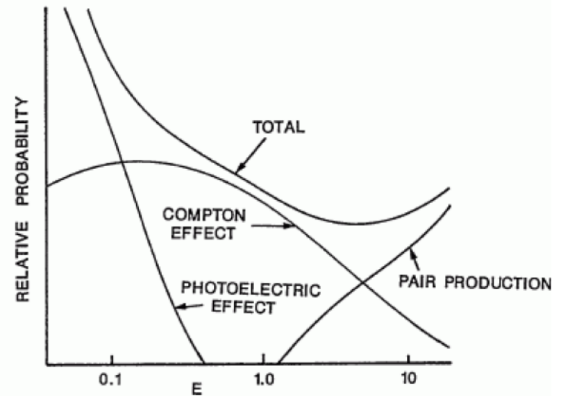
Relative probability of three processes
