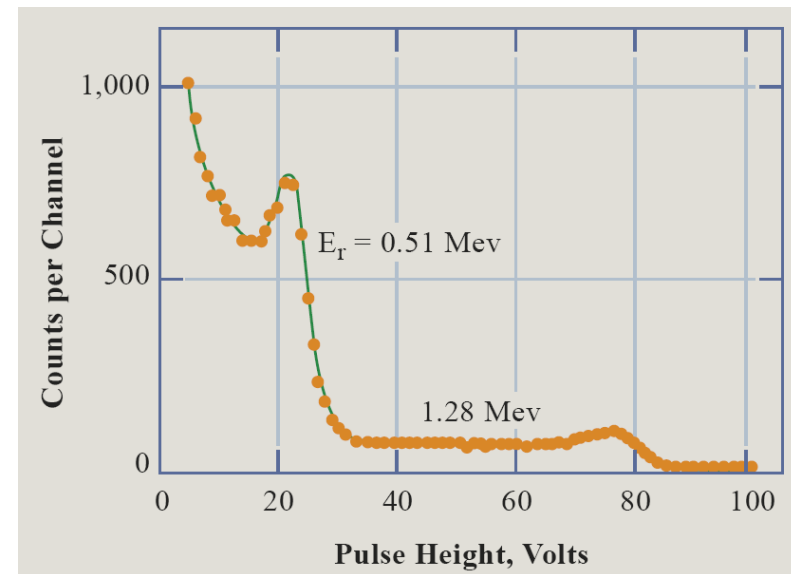
Pulse-height spectra of Compton electrons produced by 0.51- and 1.28-MeV gamma rays.
