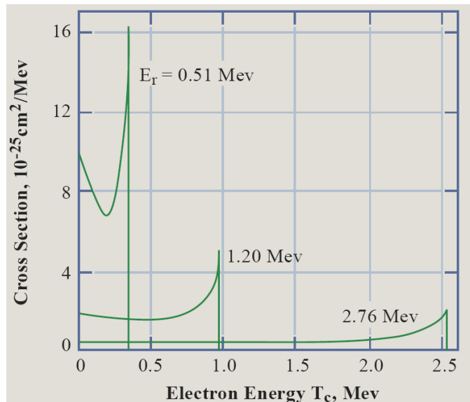
Energy distribution of Compton electrons for several incident gamma-ray energies.
