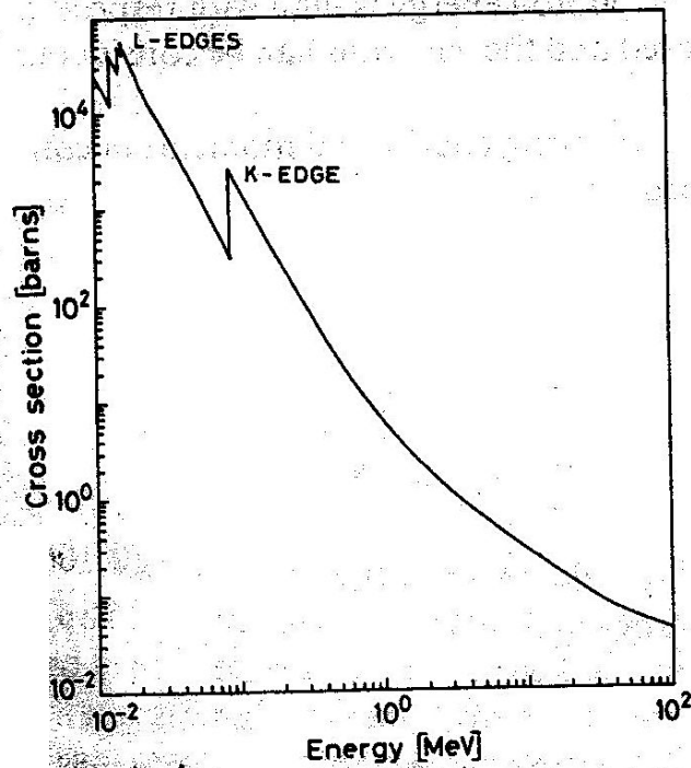
Calculated photoelectric cross section for lead
